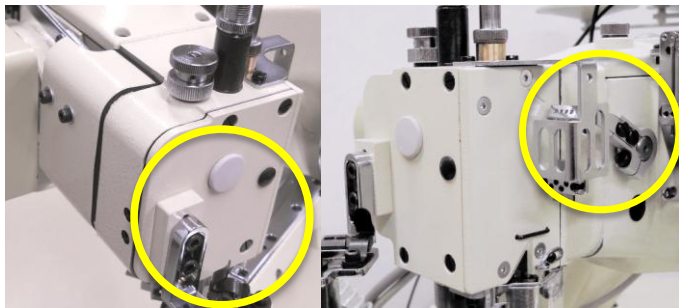
Enclosed needle drive mechanism
